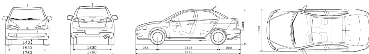
All measurements in millimetres
